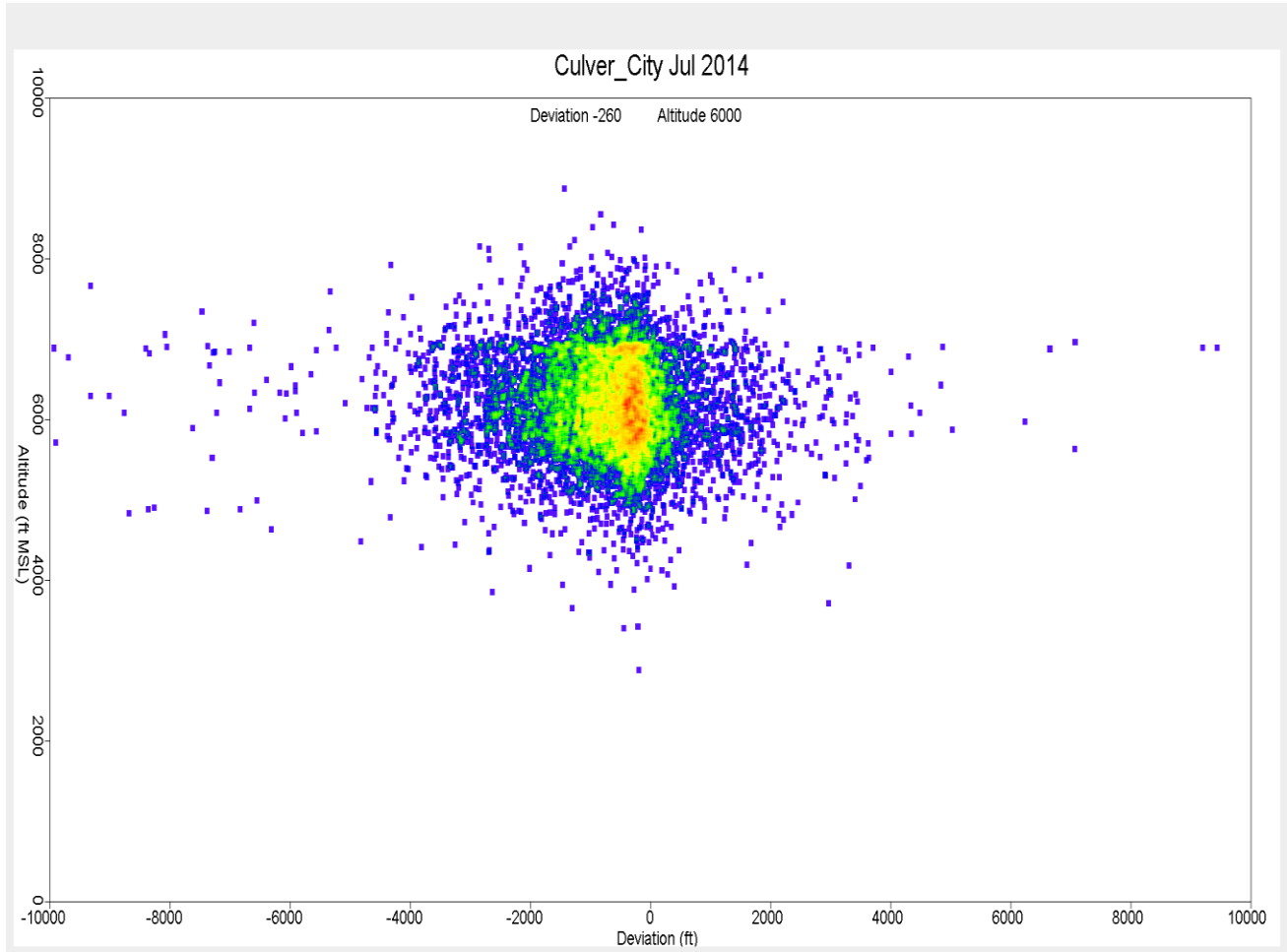
Figure 19. Altitude Distribution over Culver City July 2014
