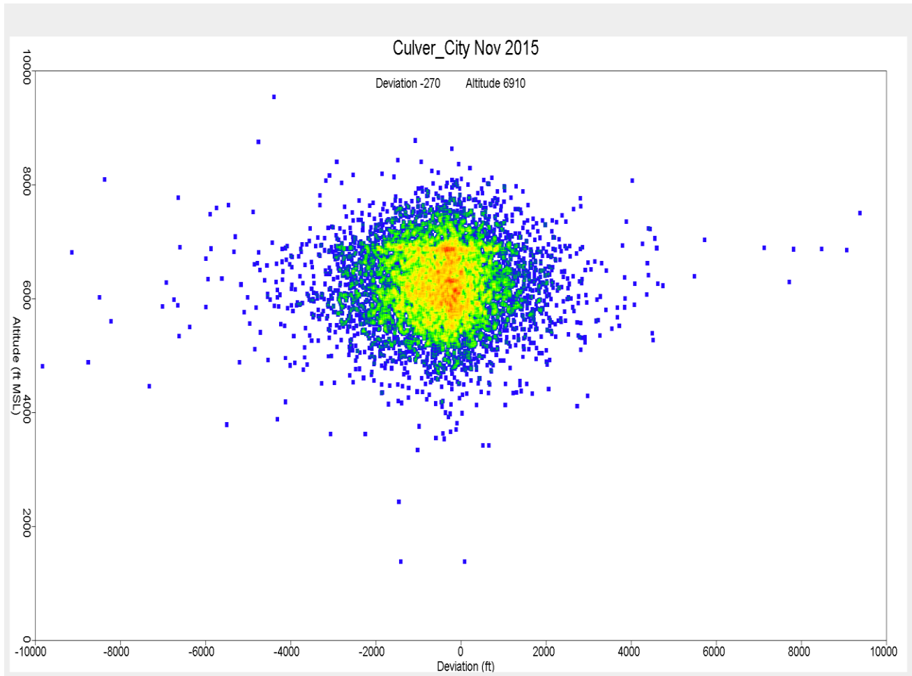
Figure 47. Altitude Distribution over Culver City November 2015
