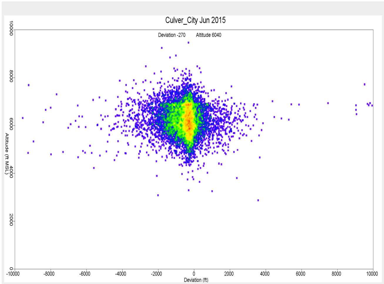
Figure 42. Altitude Distribution over Culver City June 2015
