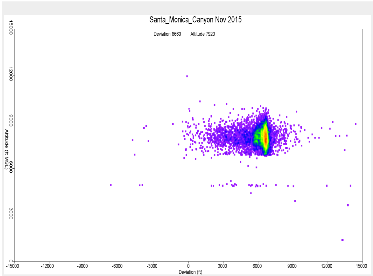
Figure 35. Altitude Distribution over Santa Monica Canyon November 2015
