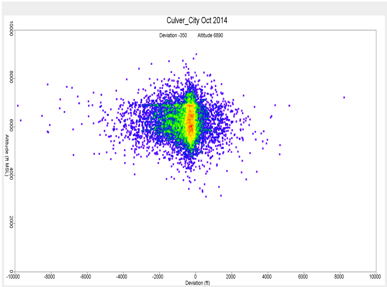
Figure 22. Altitude Distribution over Culver City October 2014
