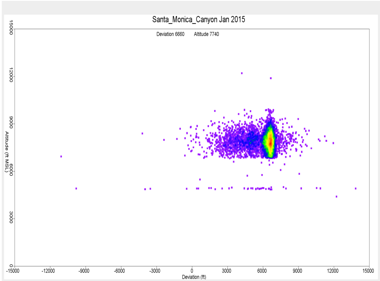
Figure 25. Altitude Distribution over Santa Monica Canyon January 2015
