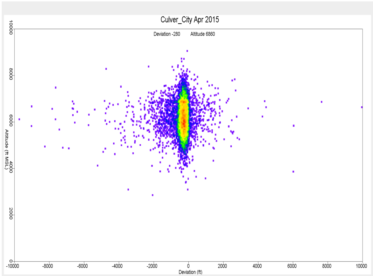
Figure 40. Altitude Distribution over Culver City April 2015
