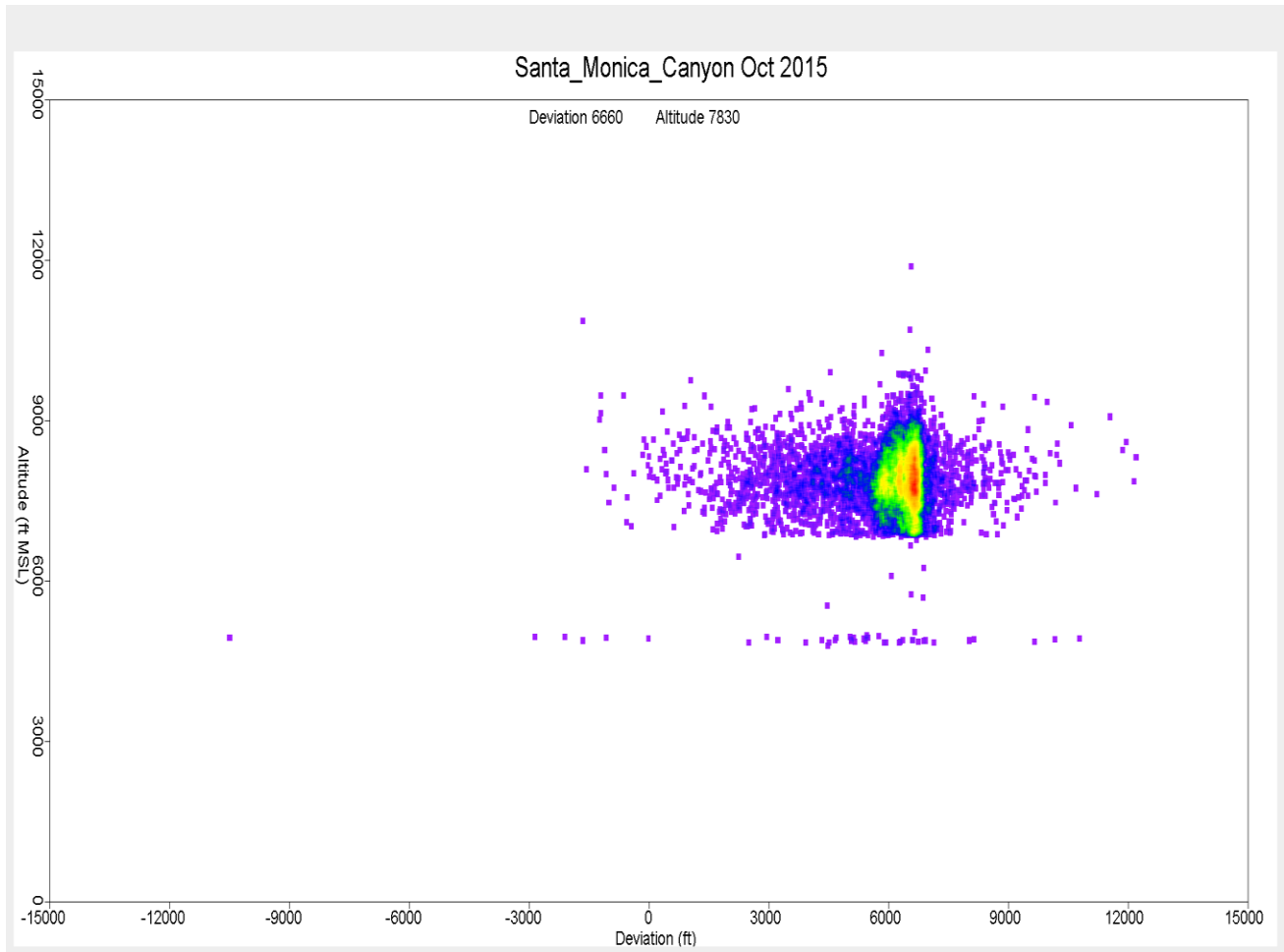
Figure 34. Altitude Distribution over Santa Monica Canyon October 2015
