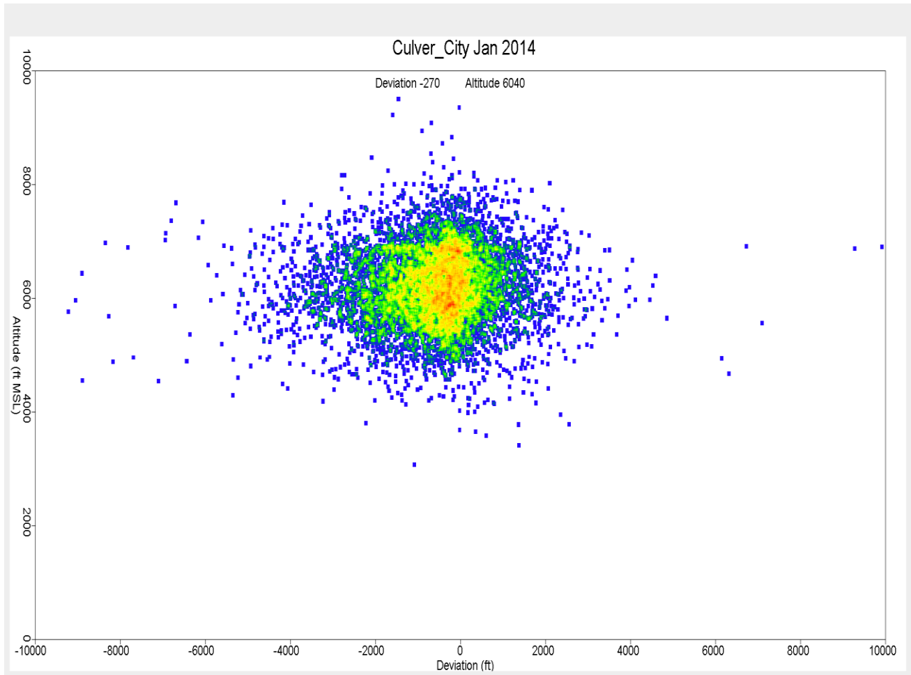
Figure 13. Altitude Distribution over Culver City January 2014
