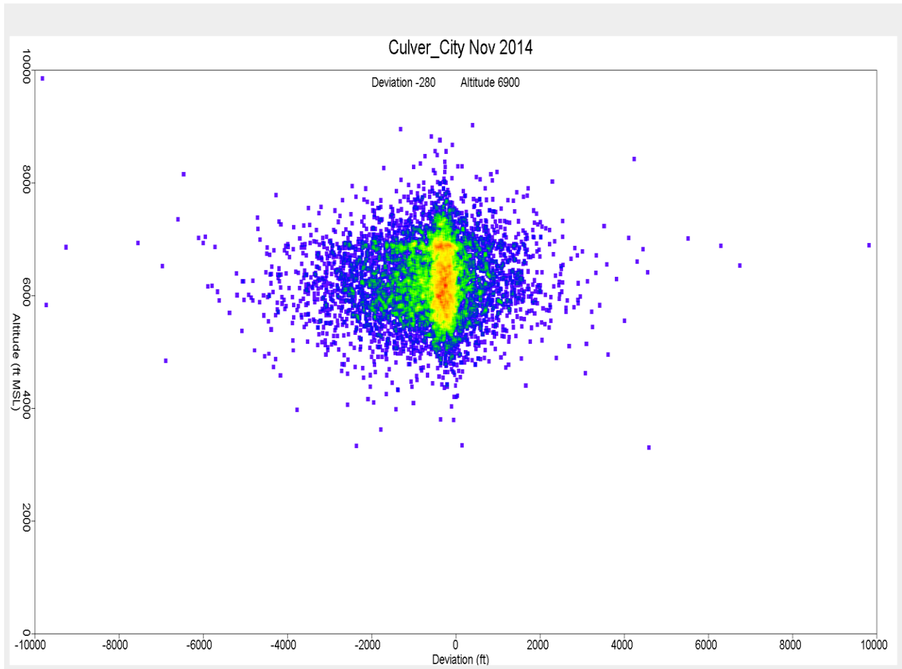
Figure 23. Altitude Distribution over Culver City November 2014
