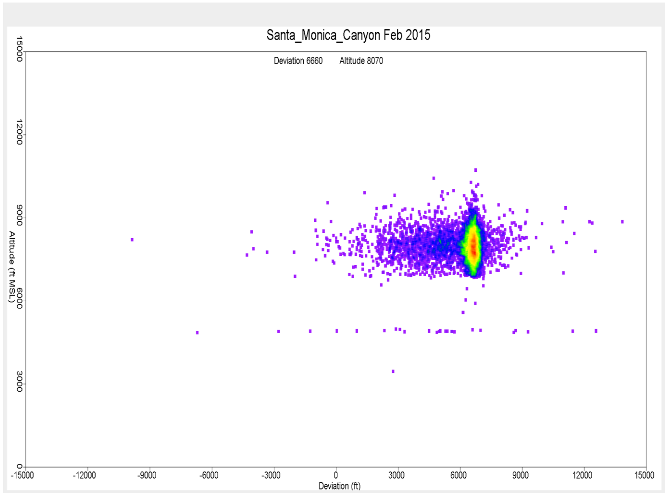
Figure 26. Altitude Distribution over Santa Monica Canyon February 2015
