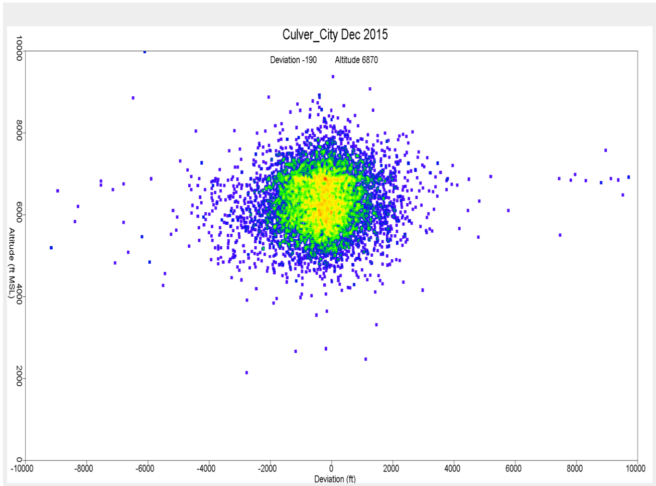
Figure 48. Altitude Distribution over Culver City December 2015
