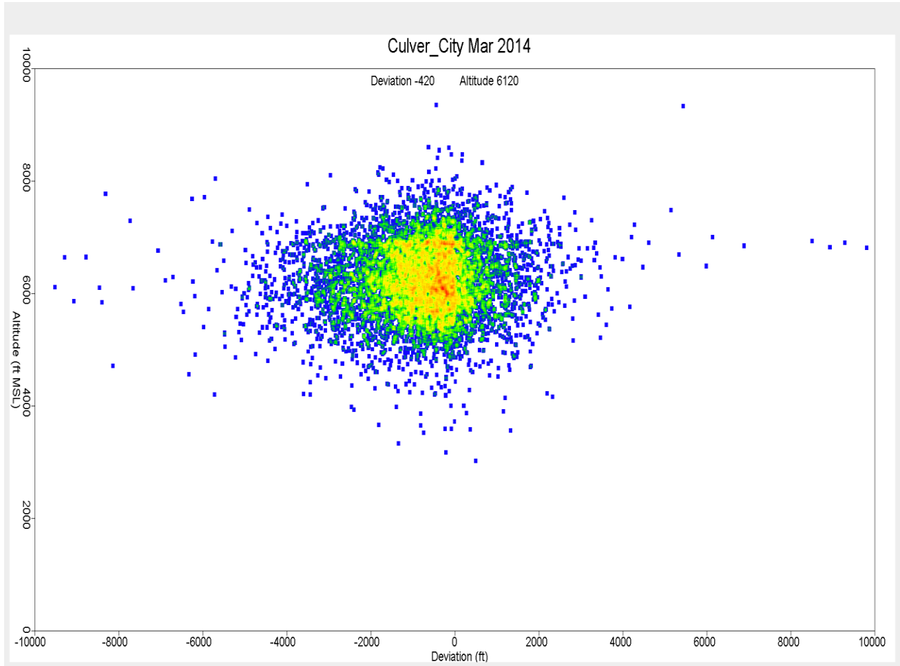
Figure 15. Altitude Distribution over Culver City March 2014
