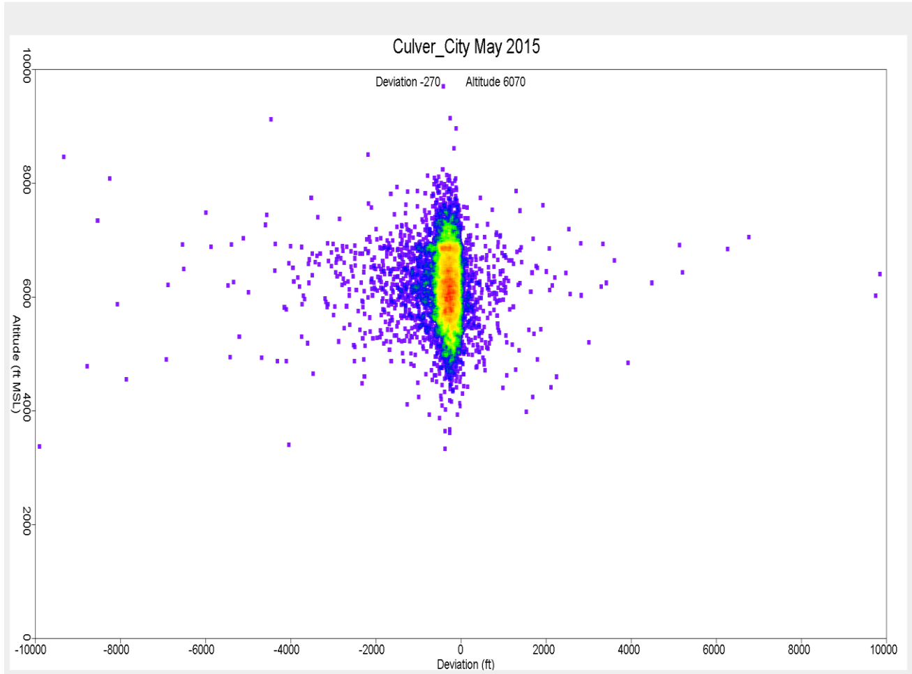
Figure 41. Altitude Distribution over Culver City May 2015
