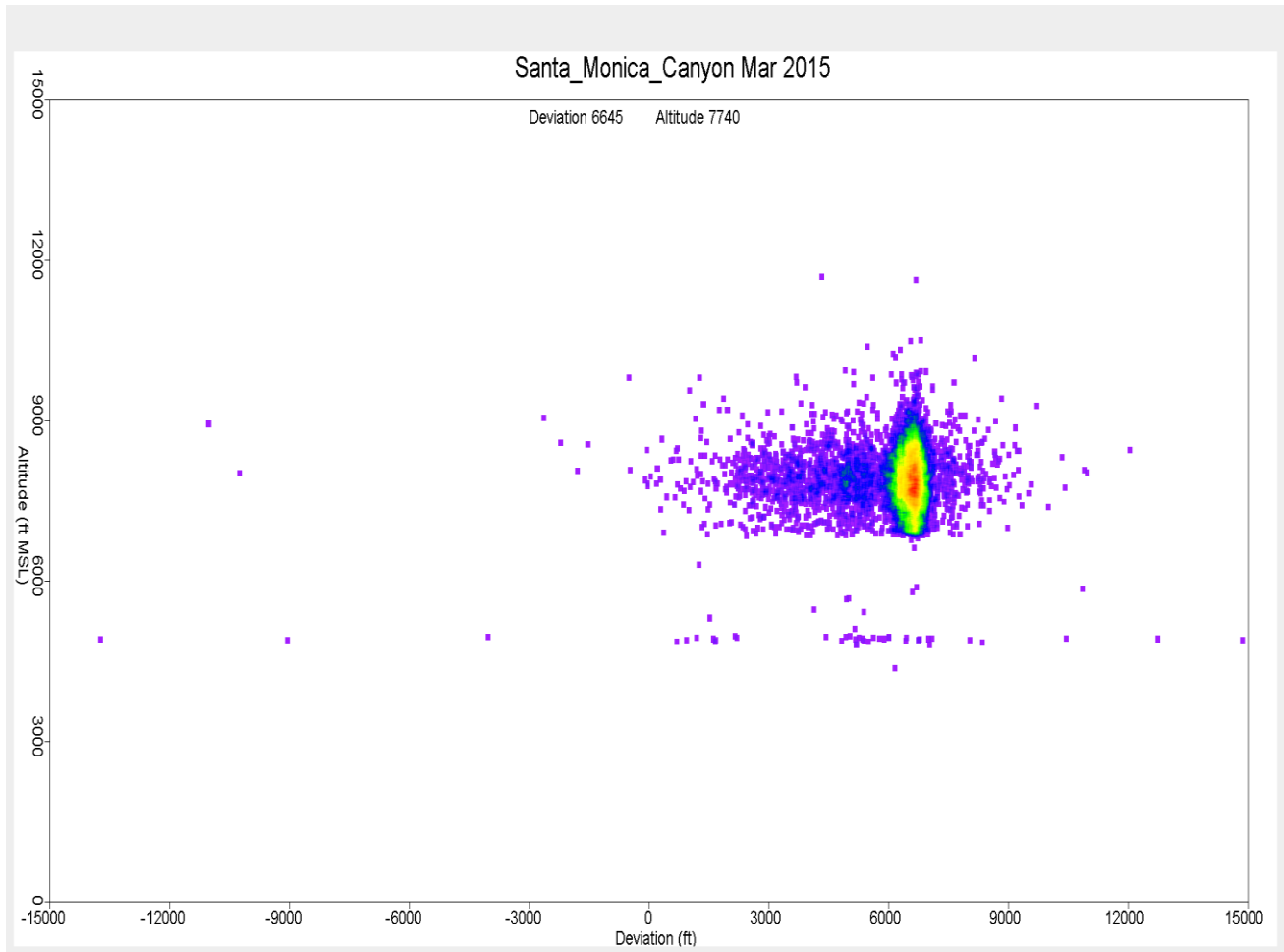
Figure 27. Altitude Distribution over Santa Monica Canyon March 2015
