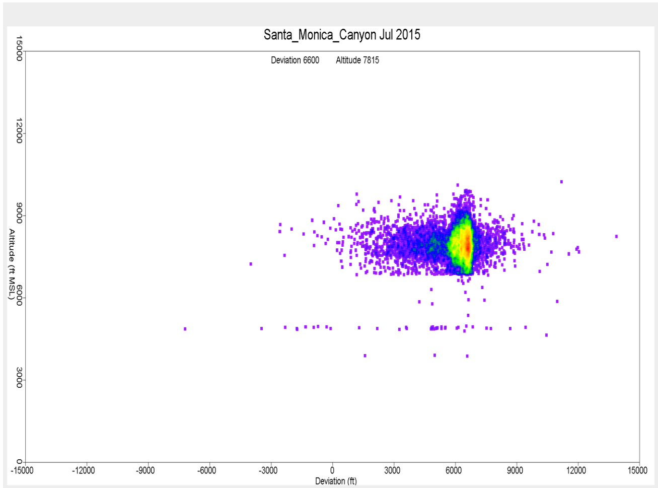
Figure 31. Altitude Distribution over Santa Monica Canyon July 2015
