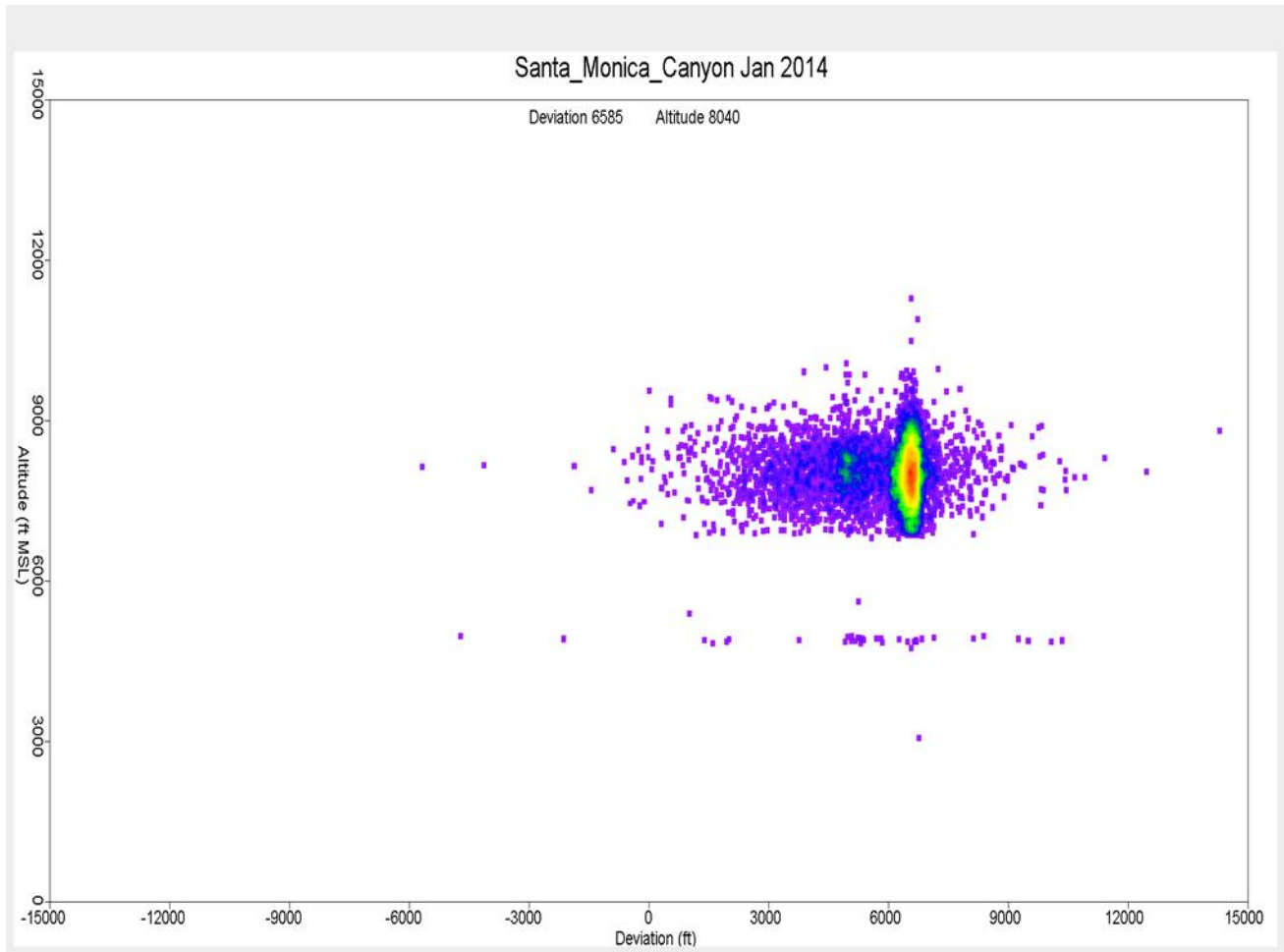
Figure 1. Altitude Distribution over Santa Monica Canyon January 2014
