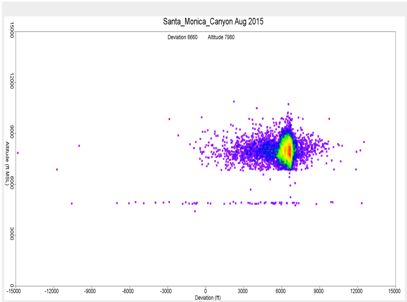
Figure 32. Altitude Distribution over Santa Monica Canyon August 2015
