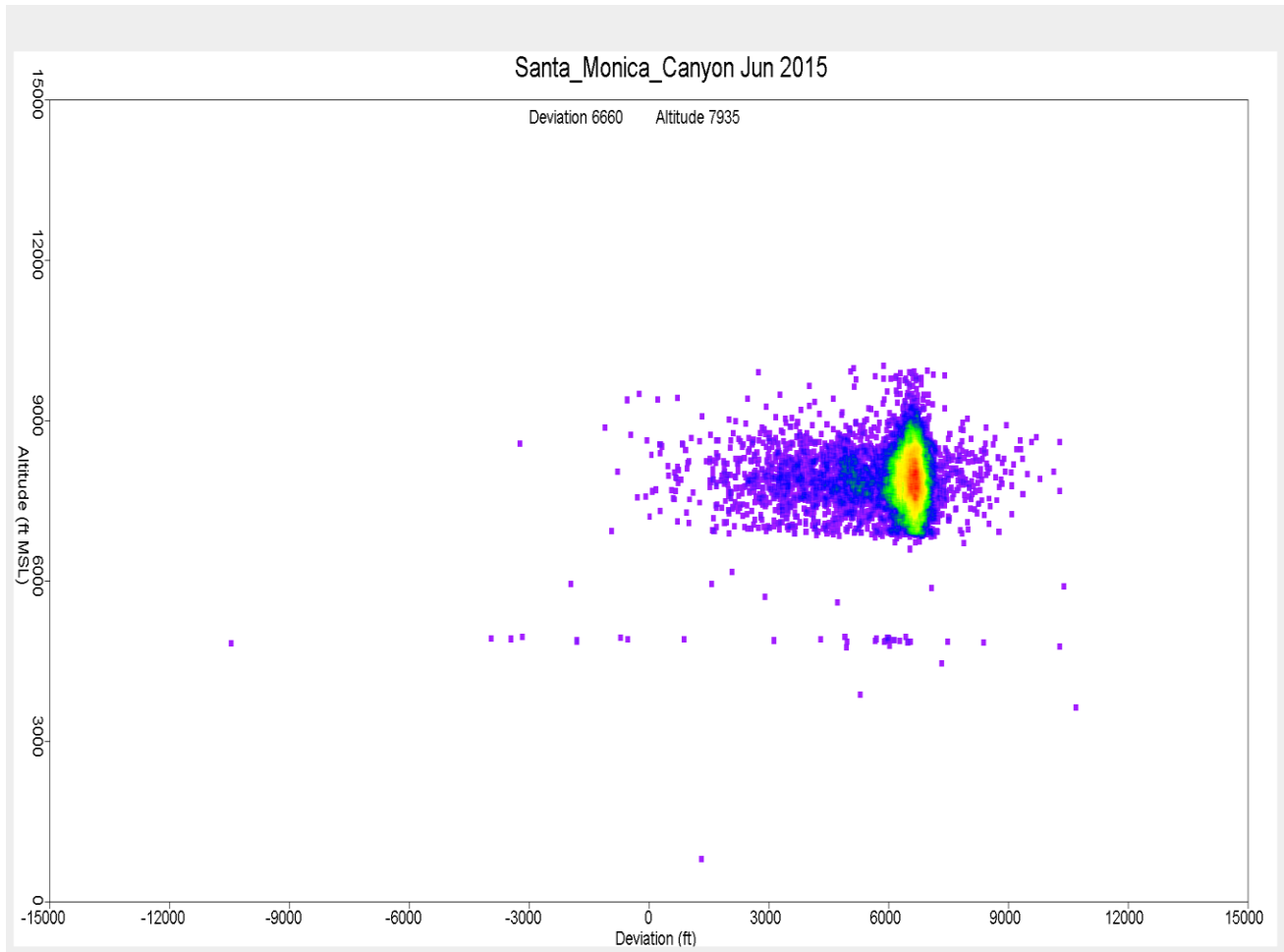
Figure 30. Altitude Distribution over Santa Monica Canyon June 2015
