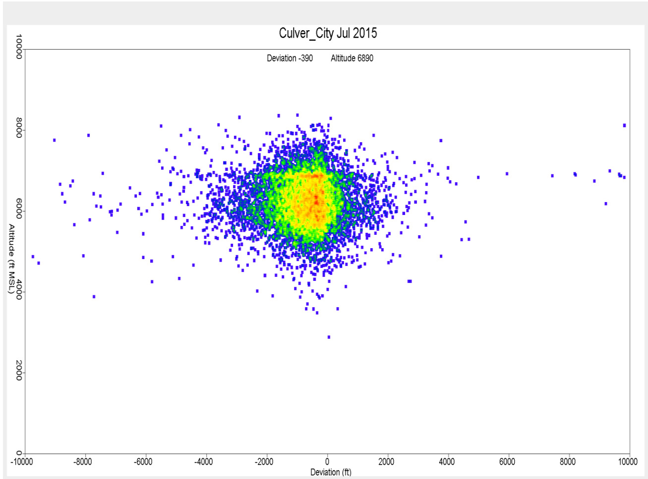
Figure 43. Altitude Distribution over Culver City July 2015
