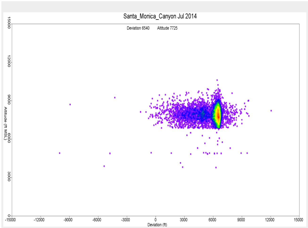
Figure 7. Altitude Distribution over Santa Monica Canyon July 2014
