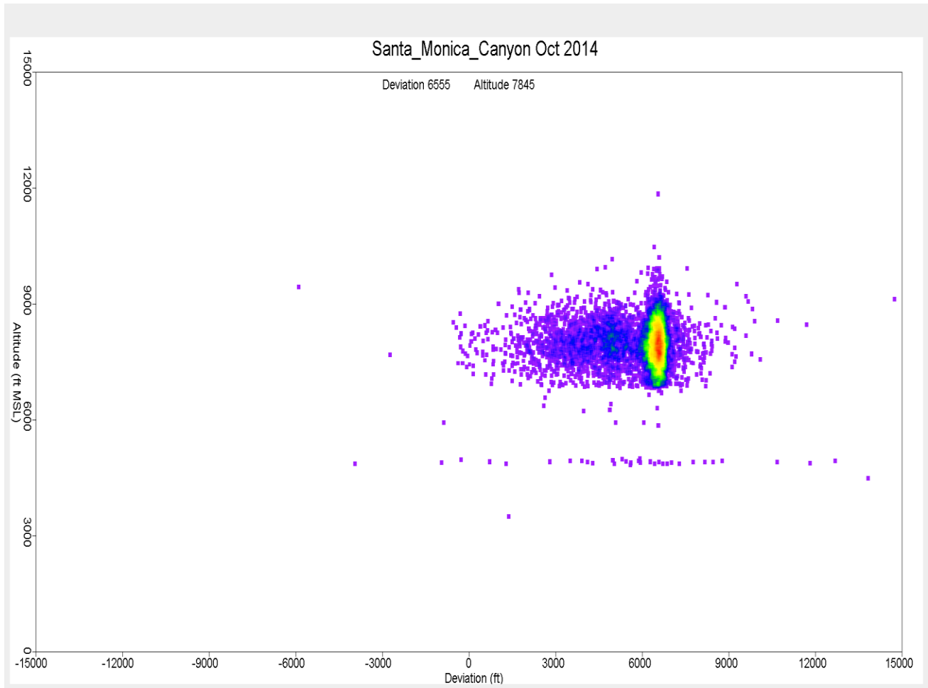
Figure 10. Altitude Distribution over Santa Monica Canyon October 2014
