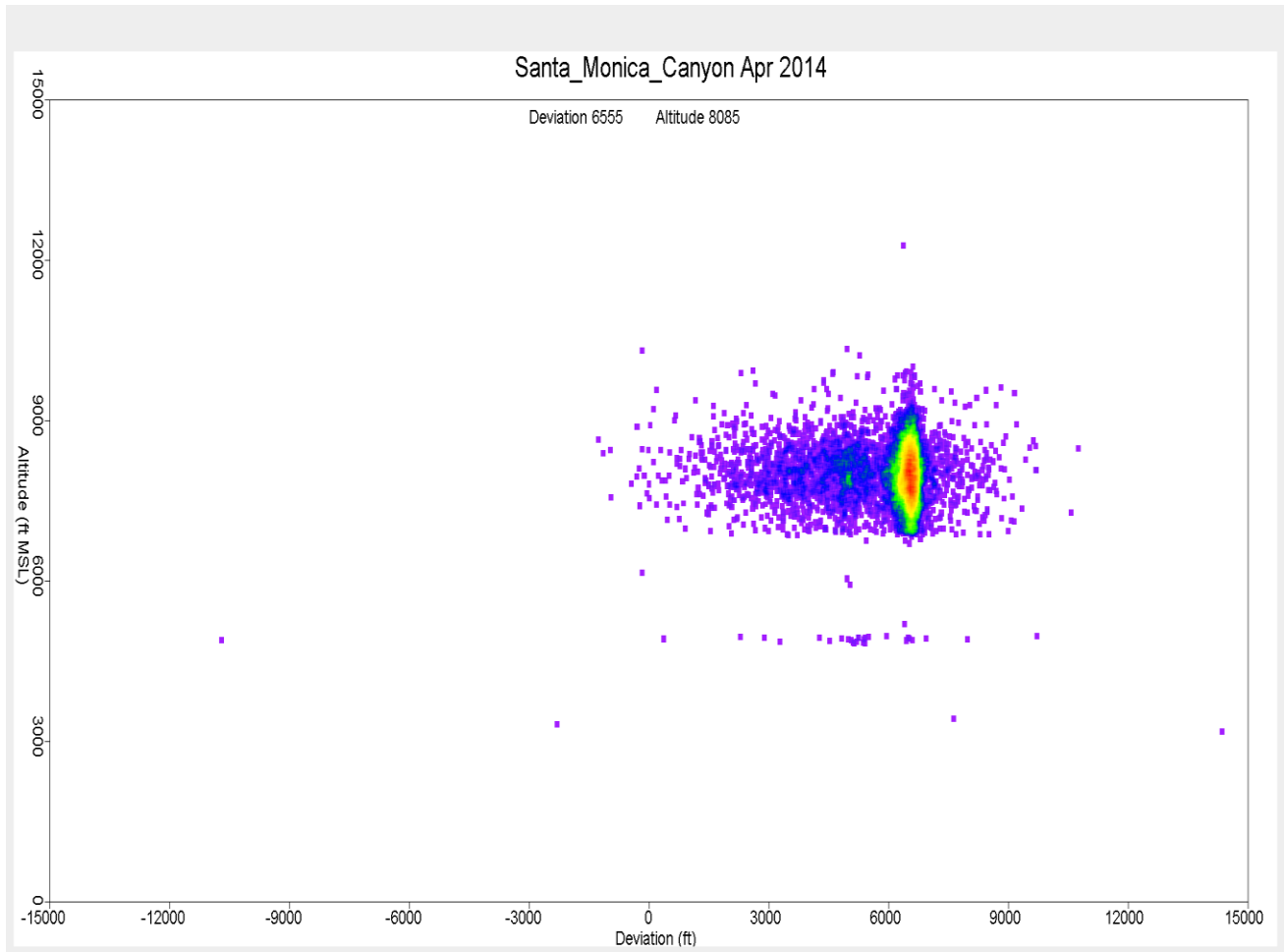
Figure 4. Altitude Distribution over Santa Monica Canyon April 2014
