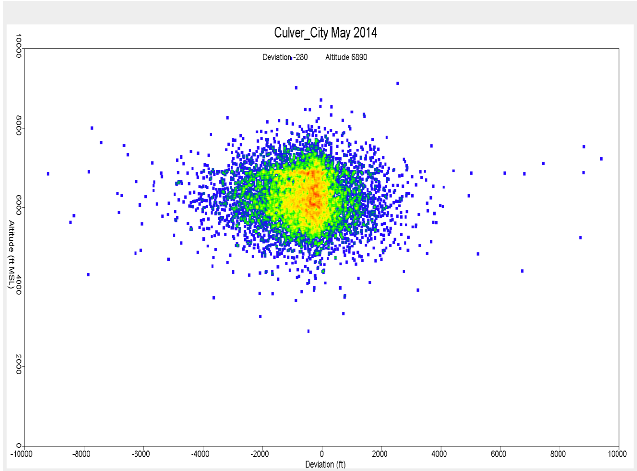
Figure 17. Altitude Distribution over Culver City May 2014
