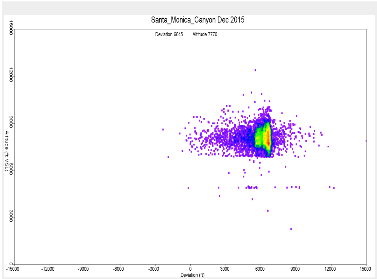
Figure 36. Altitude Distribution over Santa Monica Canyon December 2015
