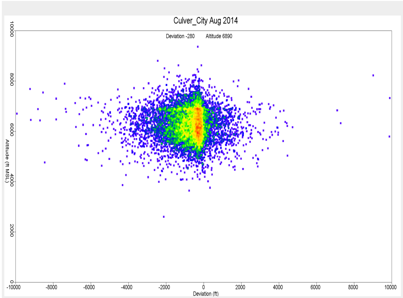
Figure 20. Altitude Distribution over Culver City August 2014
