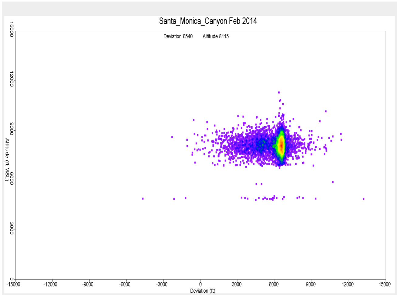
Figure 2. Altitude Distribution over Santa Monica Canyon February 2014
