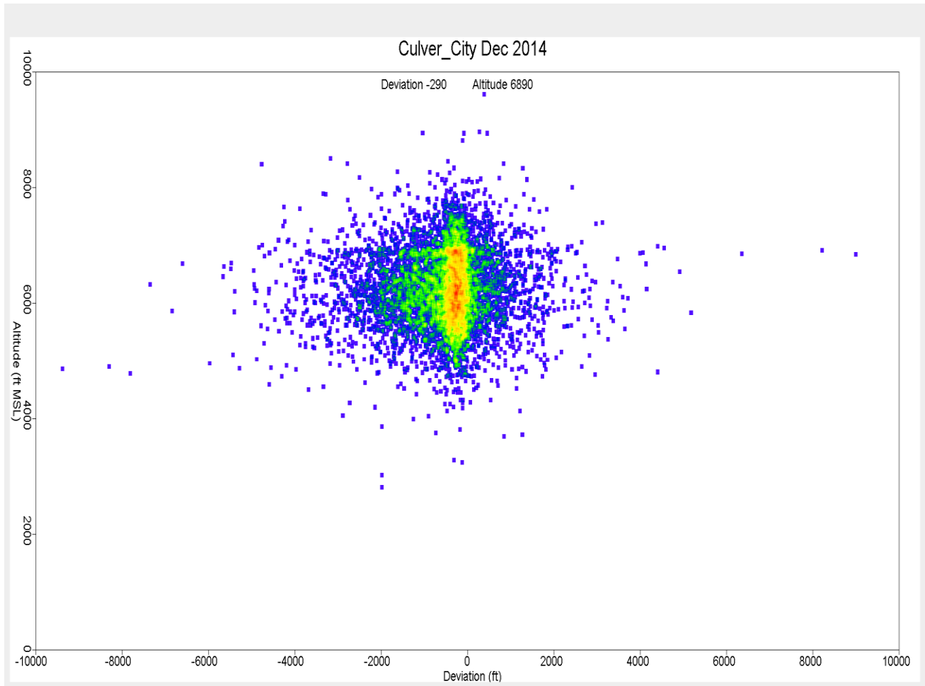
Figure 24. Altitude Distribution over Culver City December 2014
