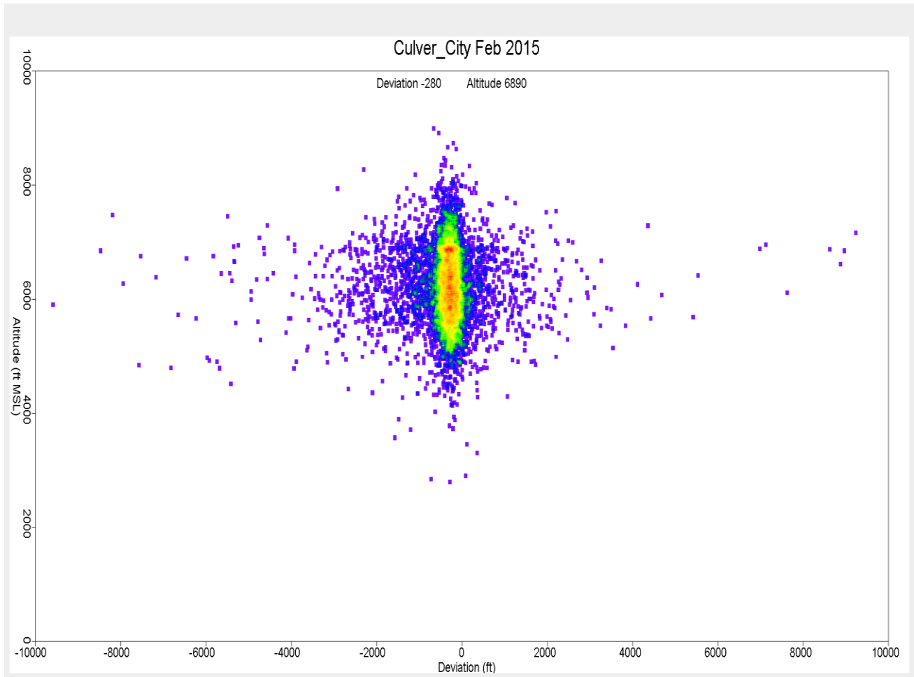
Figure 38. Altitude Distribution over Culver City February 2015
