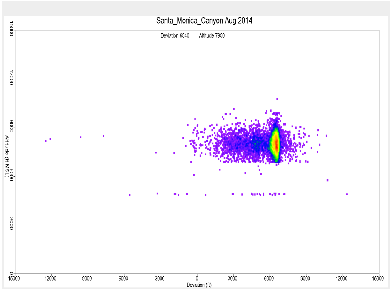
Figure 8. Altitude Distribution over Santa Monica Canyon August 2014
