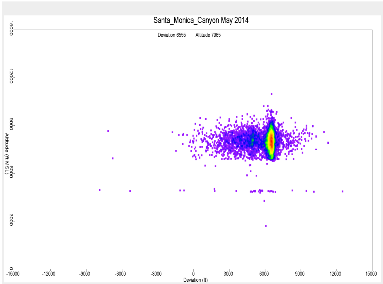
Figure 5. Altitude Distribution over Santa Monica Canyon May 2014
