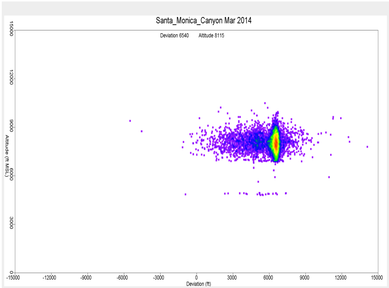
Figure 3. Altitude Distribution over Santa Monica Canyon March 2014
