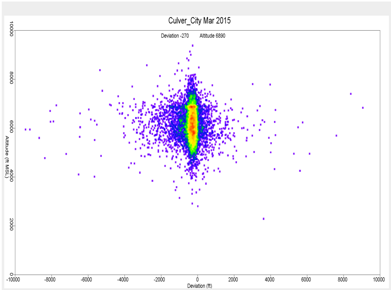
Figure 39. Altitude Distribution over Culver City March 2015
