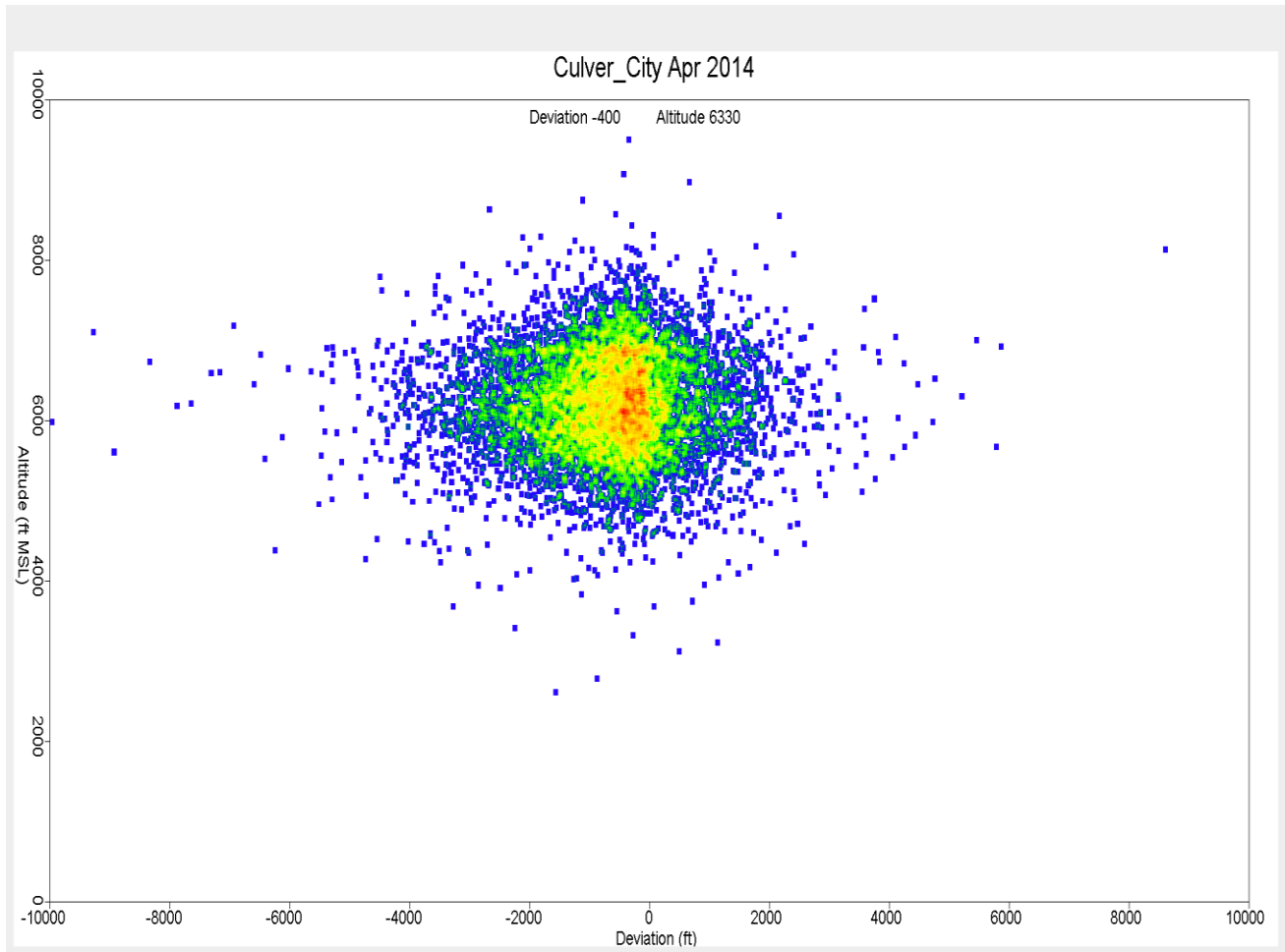
Figure 16. Altitude Distribution over Culver City April 2014
