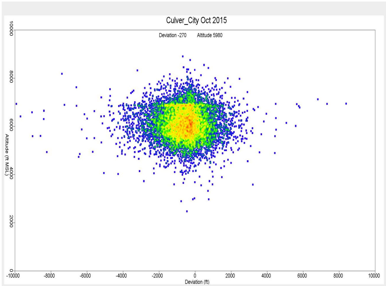
Figure 46. Altitude Distribution over Culver City October 2015
