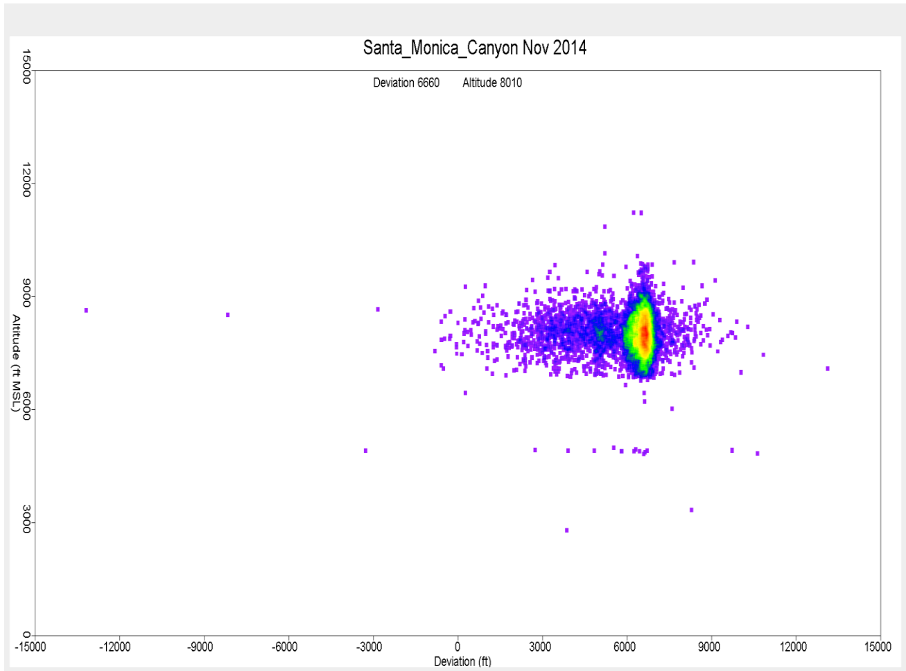
Figure 11. Altitude Distribution over Santa Monica Canyon November 2014
