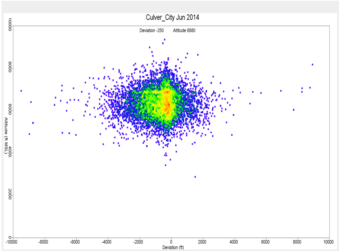
Figure 18. Altitude Distribution over Culver City June 2014
