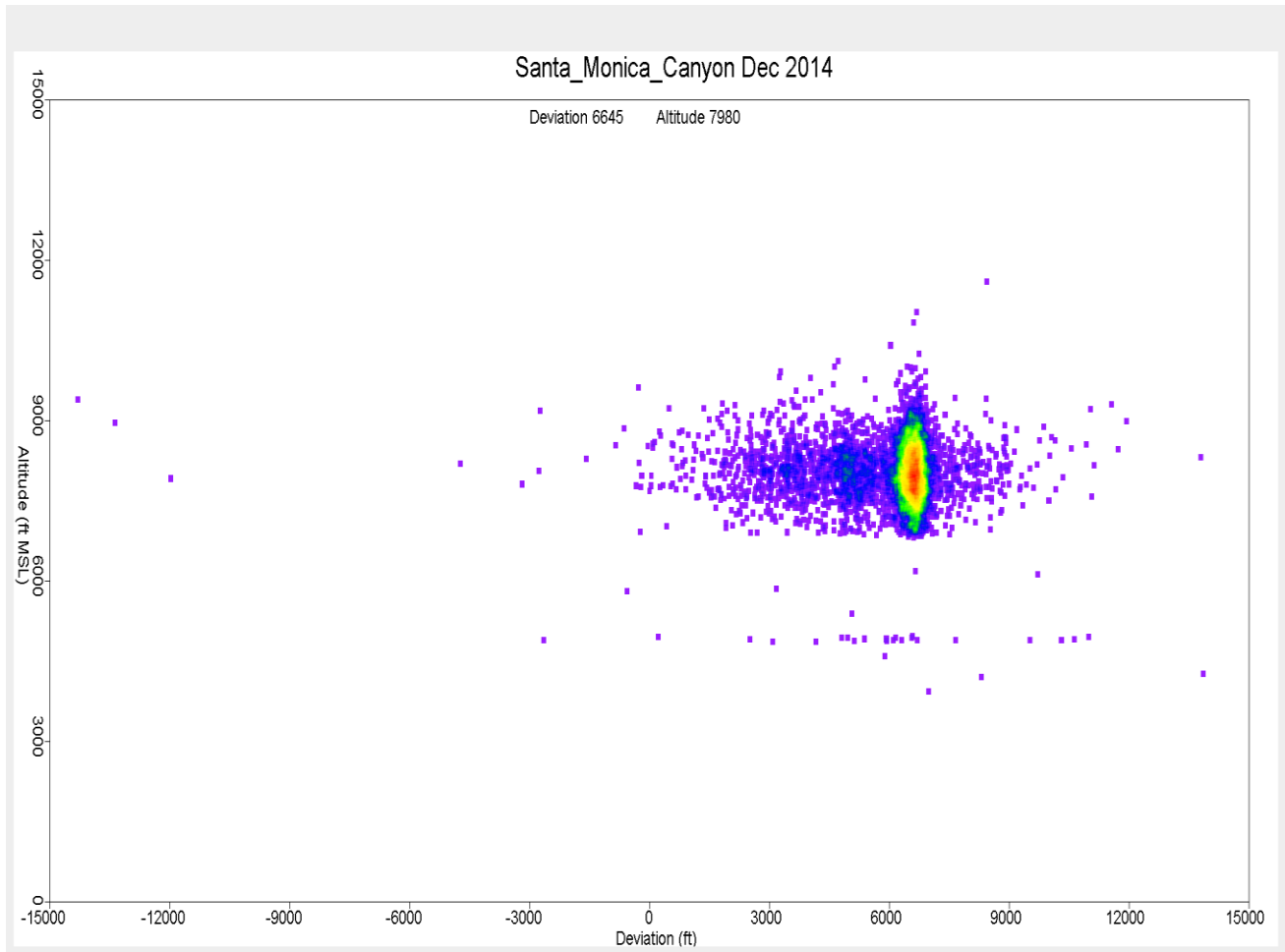
Figure 12. Altitude Distribution over Santa Monica Canyon December 2014
