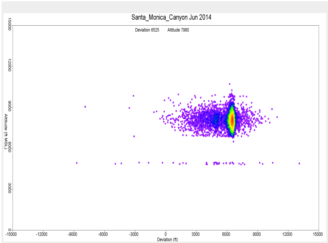
Figure 6. Altitude Distribution over Santa Monica Canyon June 2014
