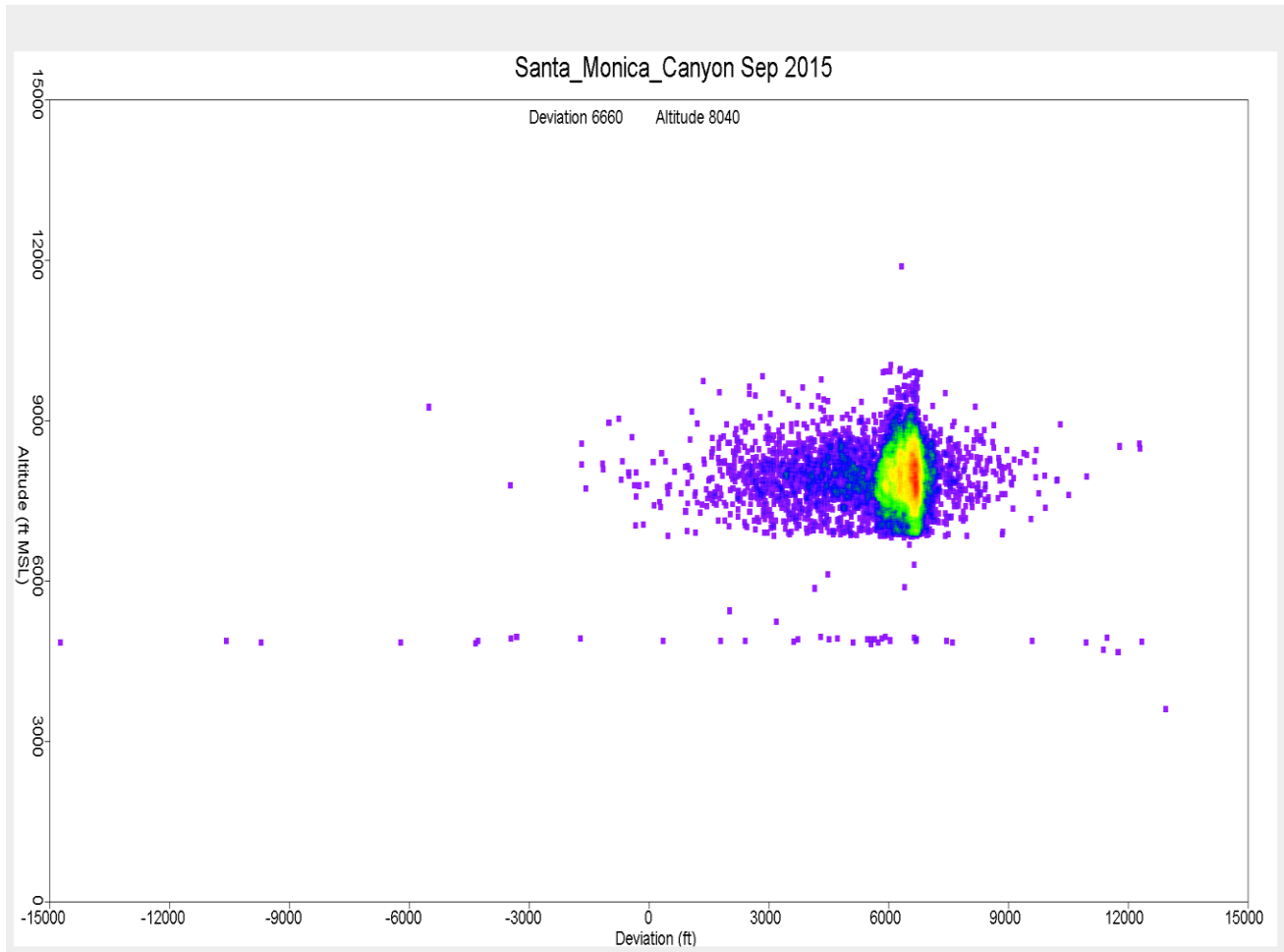
Figure 33. Altitude Distribution over Santa Monica Canyon September 2015
