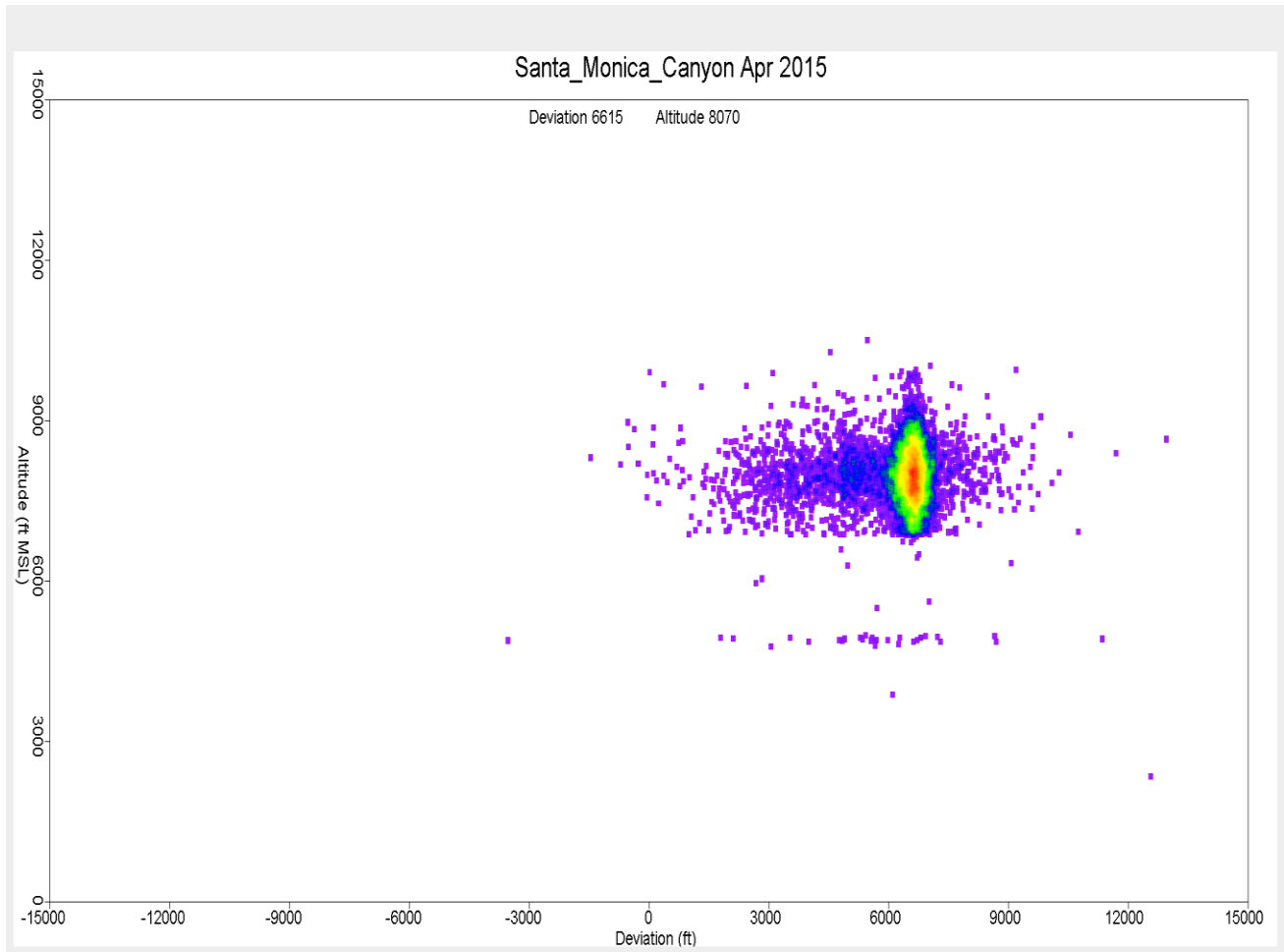
Figure 28. Altitude Distribution over Santa Monica Canyon April 2015
