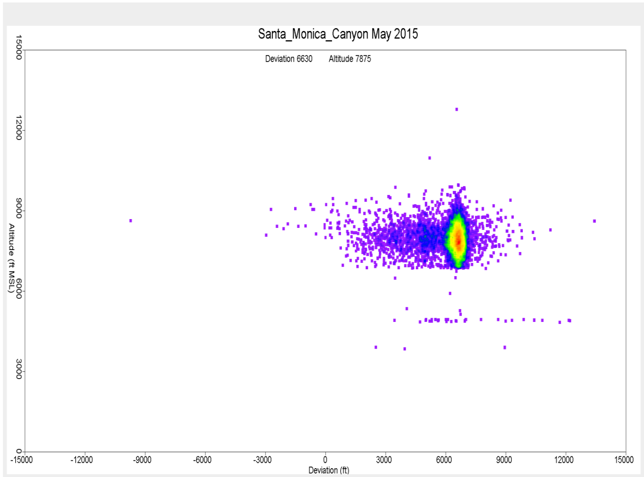
Figure 29. Altitude Distribution over Santa Monica Canyon May 2015
