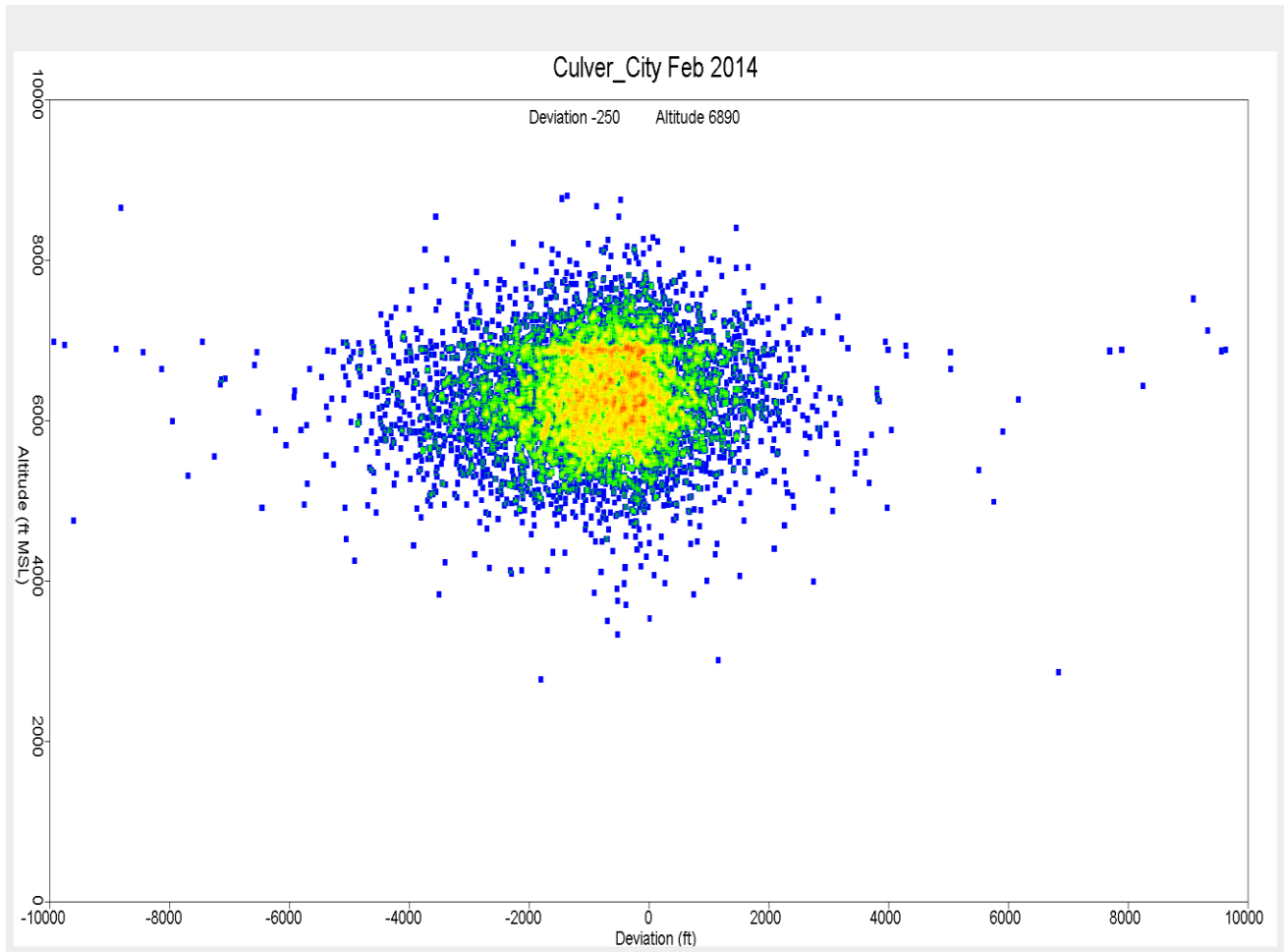
Figure 14. Altitude Distribution over Culver City February 2014
