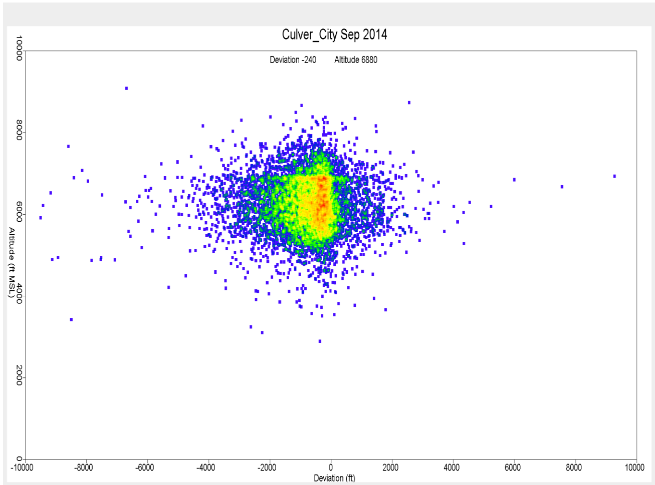
Figure 21. Altitude Distribution over Culver City September 2014
