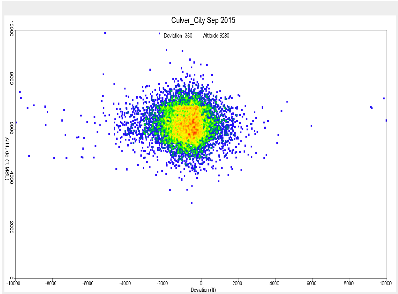
Figure 45. Altitude Distribution over Culver City September 2015
