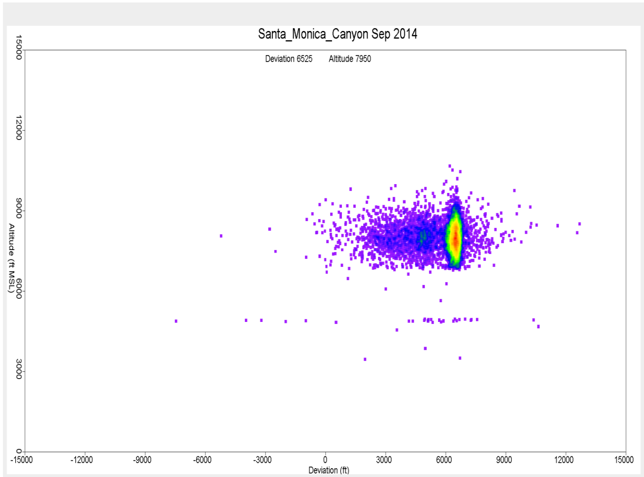
Figure 9. Altitude Distribution over Santa Monica Canyon September 2014
