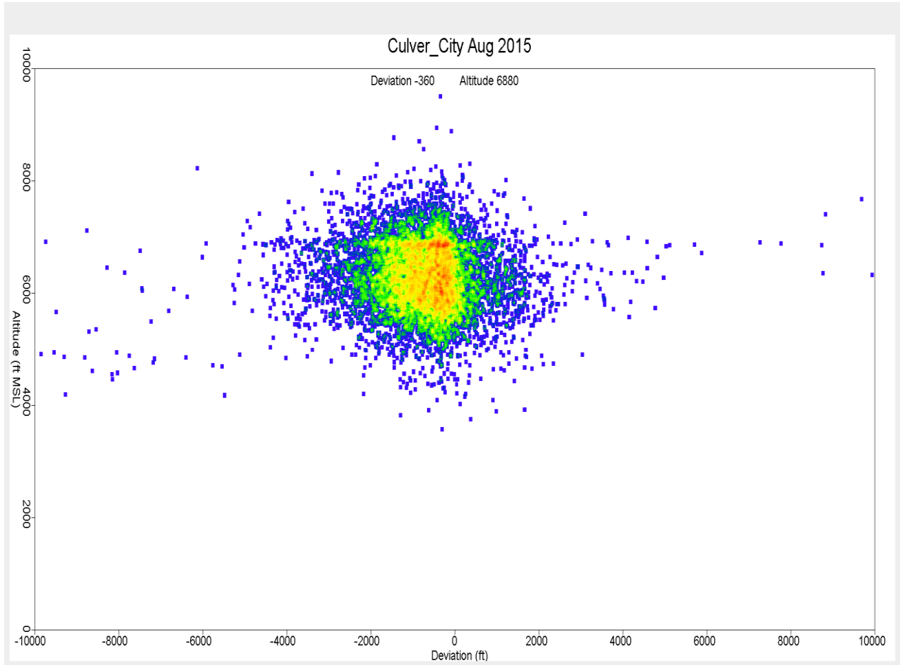
Figure 44. Altitude Distribution over Culver City August 2015
