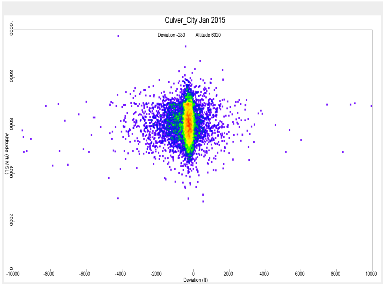
Figure 37. Altitude Distribution over Culver City January 2015
